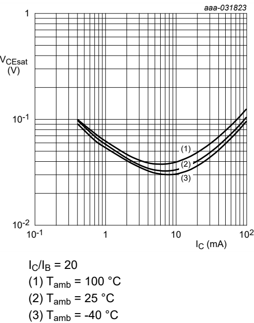
Fig. 13. NHUMH13-Q: Collector-emitter saturation voltage as a function of collector current; typical values
