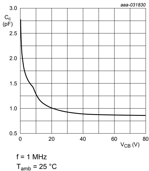
Fig. 20. NHUMH9-Q: Collector capacitance as a function of collector-base voltage; typical values
