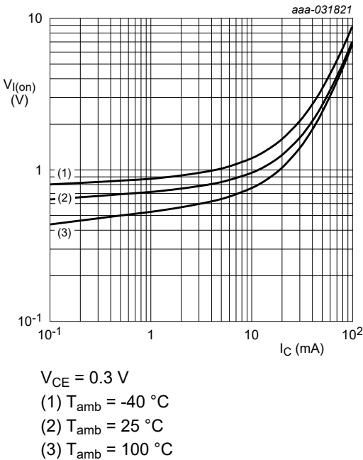
Fig. 11. NHUMH13-Q: On-state input voltage as a function of collector current; typical values
