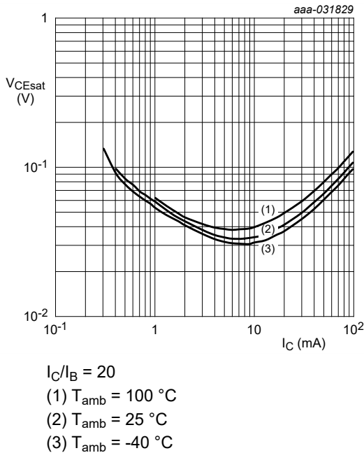
Fig. 19. NHUMH9-Q: Collector-emitter saturation voltage as a function of collector current; typical values
