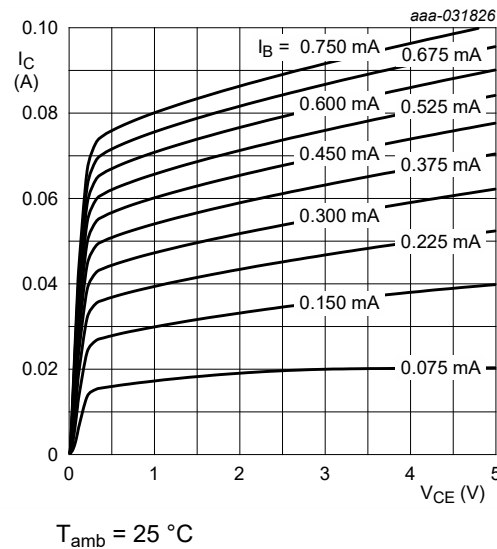
Fig. 16. NHUMH9-Q: Collector current as a function of collector-emitter voltage; typical values
