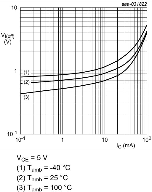
Fig. 12. NHUMH13-Q: Off-state input voltage as a function of collector current; typical values
