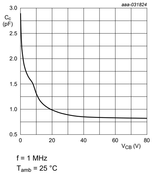
Fig. 14. NHUMH13-Q: Collector capacitance as a function of collector-base voltage; typical values
