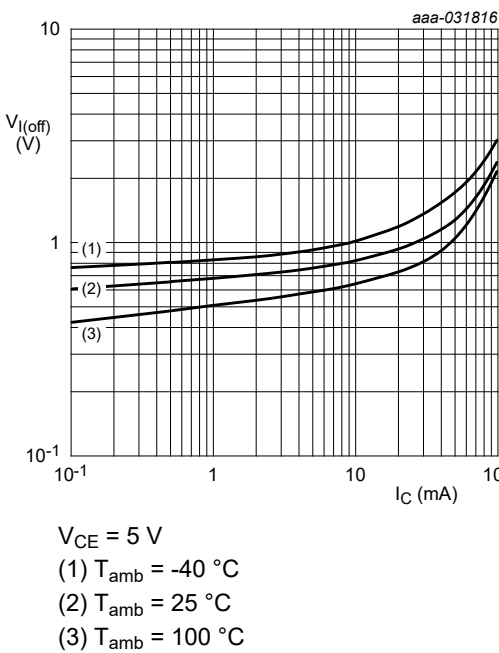
Fig. 6. NHUMH10-Q: Off-state input voltage as a function of collector current; typical values
