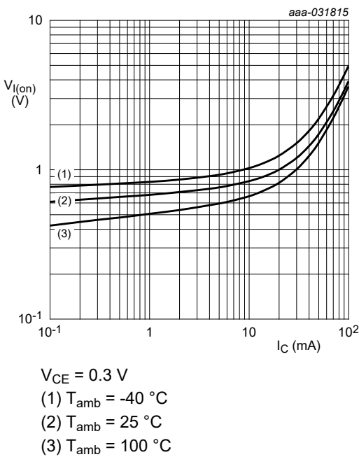
Fig. 5. NHUMH10-Q: On-state input voltage as a function of collector current; typical values
