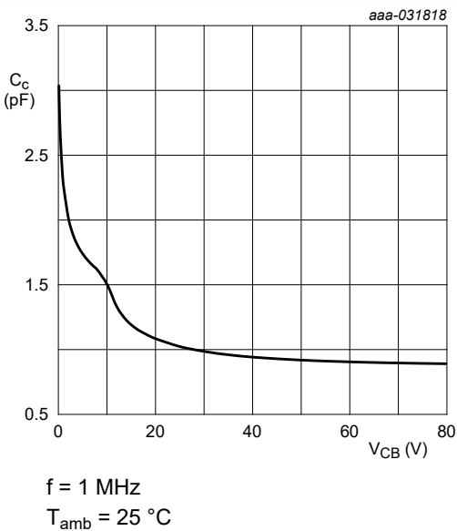
Fig. 8. NHUMH10-Q: Collector capacitance as a function of collector-base voltage; typical values
