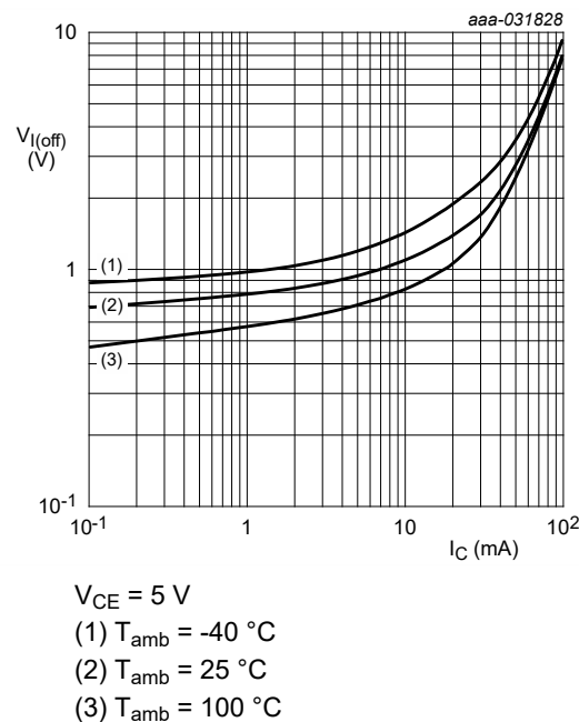
Fig. 18. NHUMH9-Q: Off-state input voltage as a function of collector current; typical values
