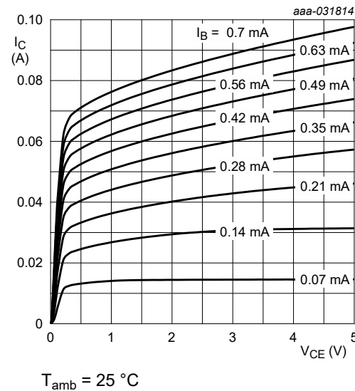
Fig. 4. NHUMH10-Q: Collector current as a function of collector-emitter voltage; typical values
